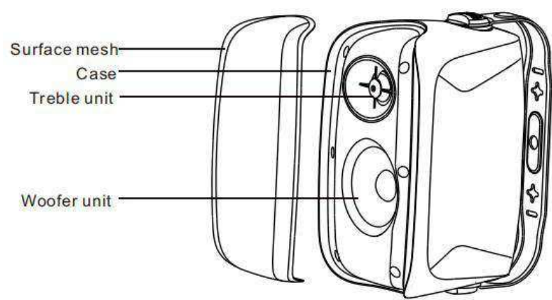
Product Exploded View
