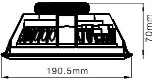
Outline Dimension
